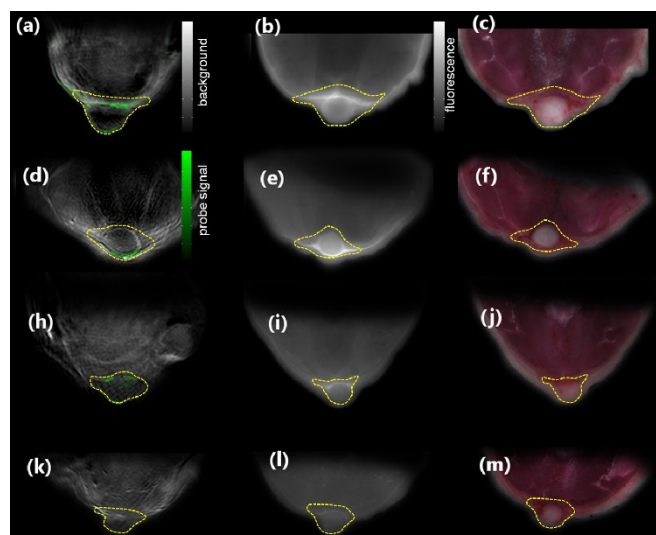
Figure 3 Imaging of targeted apoptotic marker (PSS-794) in 4 T1 tumor-bearing mice. In the first column, the MSOT images are shown. Images (a) and (d) show superposition of a single-wavelength (anatomical) optoacoustic image (in gray scale) and the unmixed component corresponding to the PSS-794 signal in color for the two mice imaged 24 h after injection. (h) shows the unmixed PSS-794 signal for the mouse imaged 3 h post injection, and (k) the ICG signal also imaged 3 h post injection. The second column shows the corresponding epi-fluorescence images of cryo-slices through the tumor. Color photograph of cryo-slices are shown in the third column. The tumor area is delineated in yellow.
