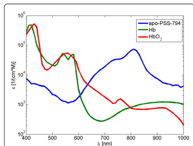
Figure 2 Molar extinction coefficient of PSS-794. In 35 mg/ml albumin along with extinction spectra of oxygenized and deoxygenized hemoglobin.
