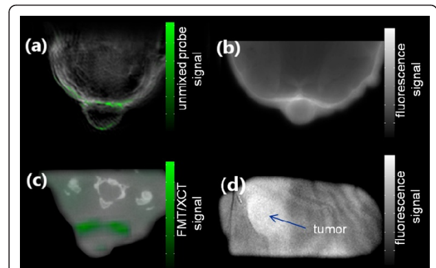
Figure 4 Comparison between optical imaging and MSOT. Image (a) shows the MSOT image, and (b) the corresponding epi-fluorescence image. An FMT-XCT reconstruction is shown in (c) and a planar transillumination image in (d)
