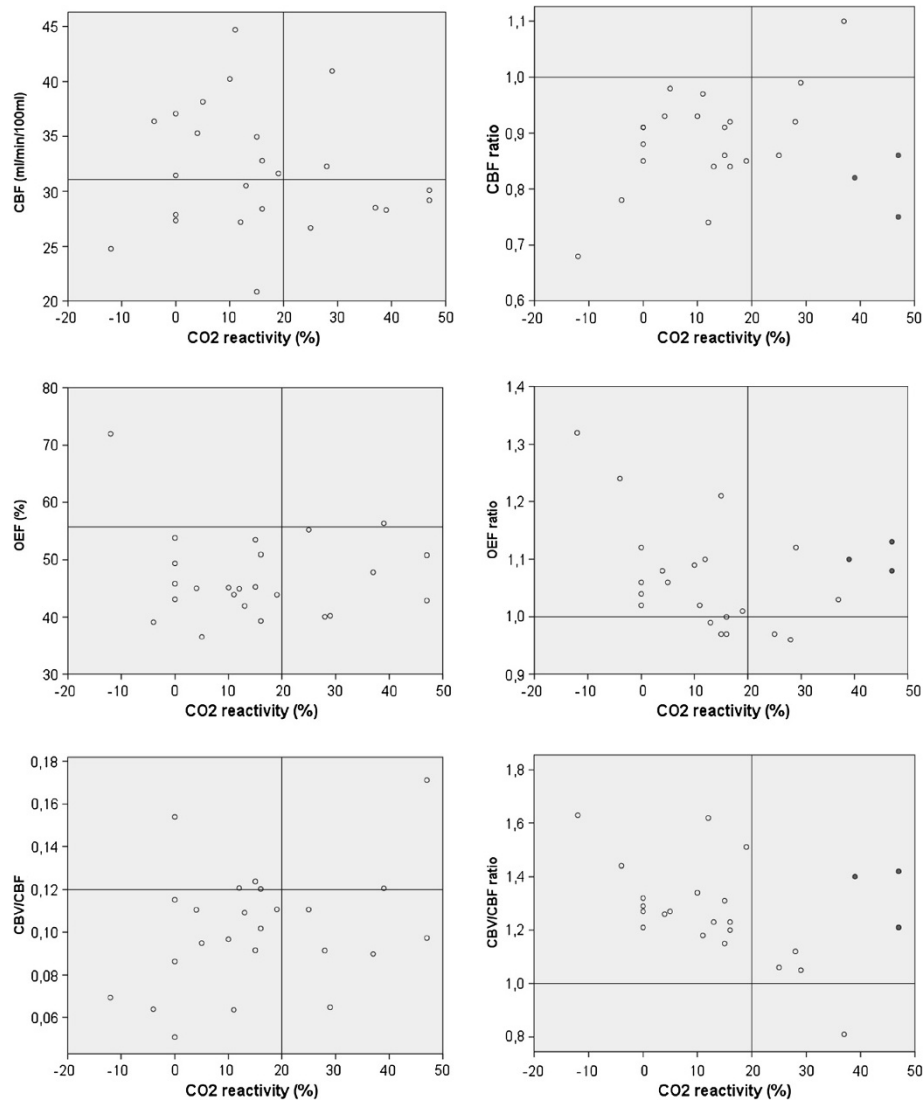
Figure 2 Relationship of CO 2 -reactivity with PET values. Scatter plots showing the relationships of CO 2 -reactivity with CBF (upper panel), OEF (middle panel), and CBV/CBF (lower panel). Within each panel, absolute values are shown on the left and ipsilateral/contralateral ratios on the right. The grey dots in the panels on the right indicate the three outliers.
